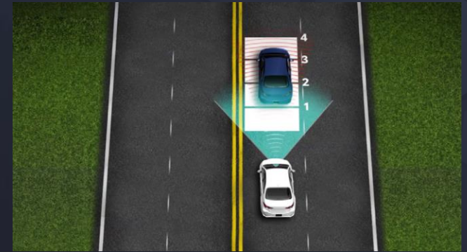
ACC (ADAPTIVE CRUISE CONTROL) EDSS (EMERGENCY DRIVING STOP SYSTEM)
